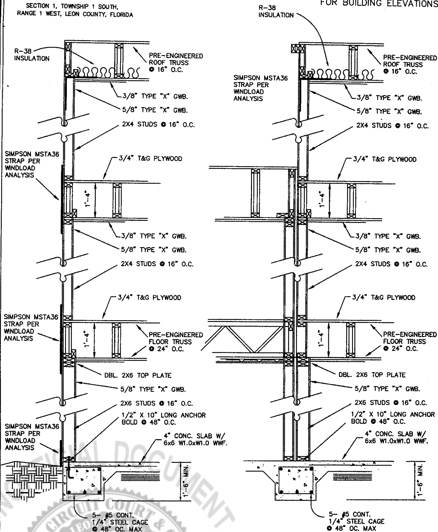
SECTION 1 INTERIOR WALL SECTION
